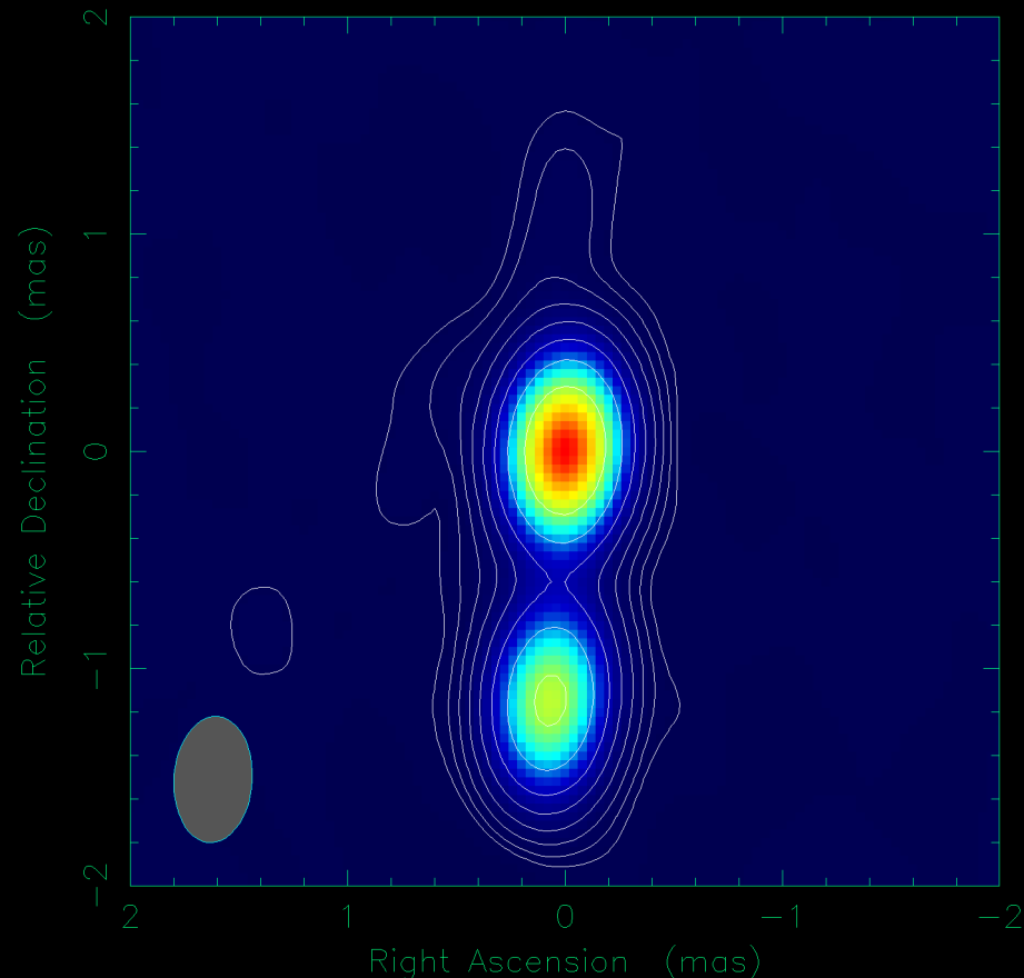
Clean I map. Array: VLBA Correlator J0137+3309 at 24.552 GHz 2019 Feb 25
