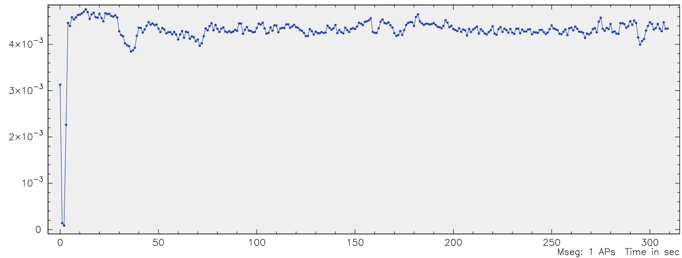
X-band fringe amplitude for NRA0530 at HN-VLBA /SC-VLBA in BG221B
