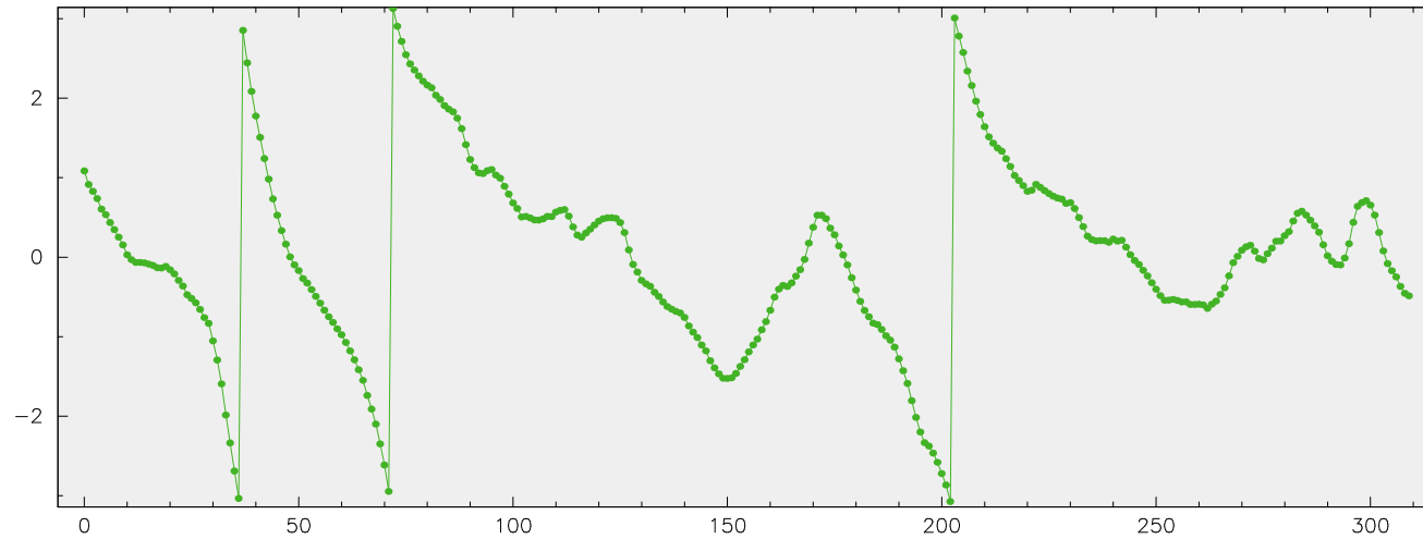
X-band fringe phase for NRA0530 at HN-VLBA /SC-VLBA in BG221B
