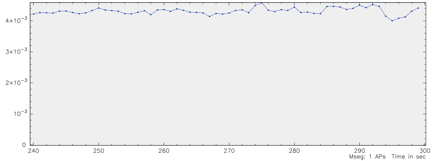
X-band fringe amplitude for NRA0530 at HN-VLBA /SC-VLBA in BG221B
