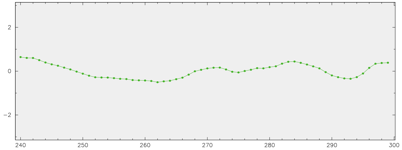
X-band fringe phase for NRA0530 at HN-VLBA /SC-VLBA in BG221B
