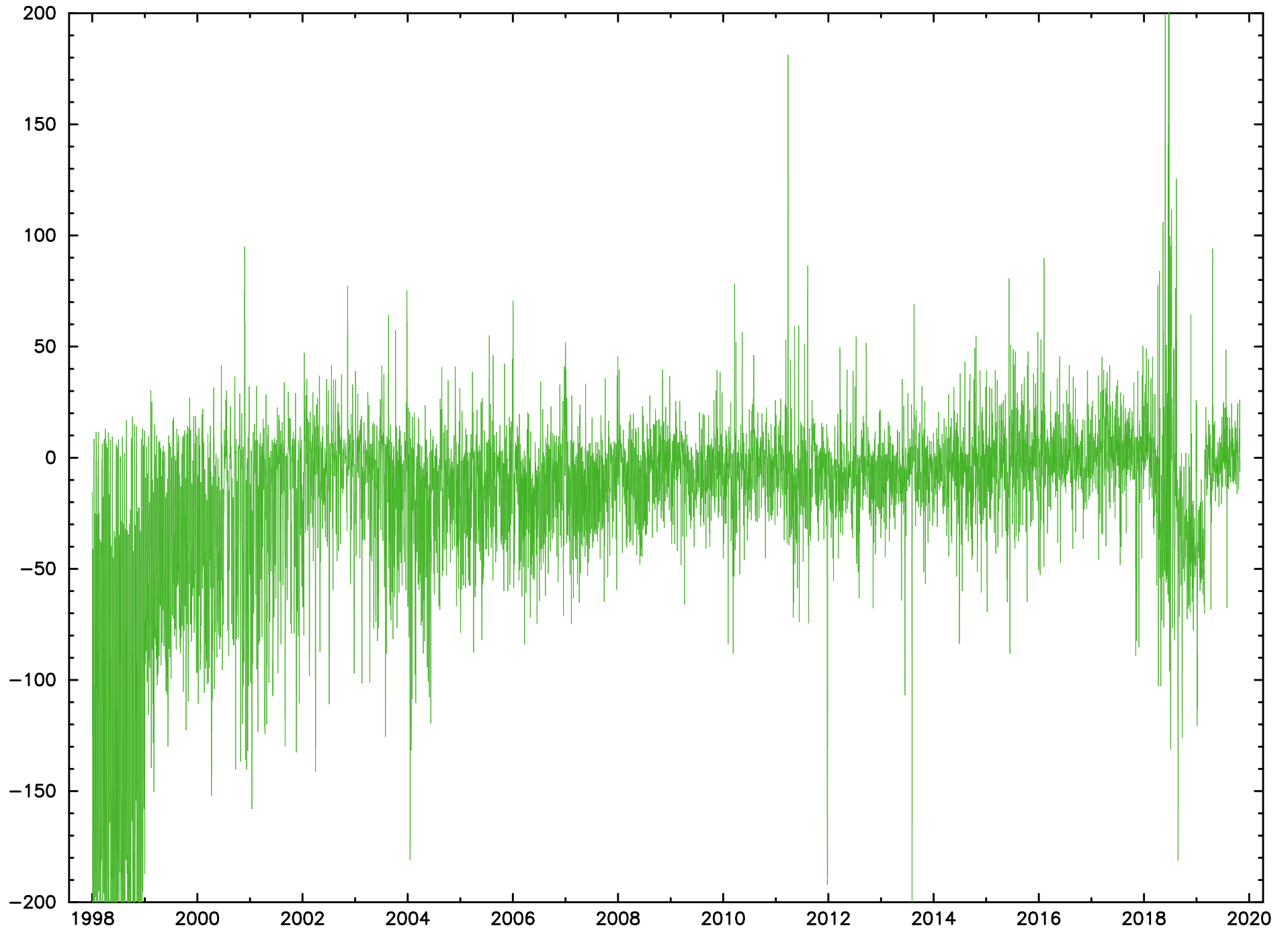
Differences IERS C04 versus USNO FINALS UT1 msec
