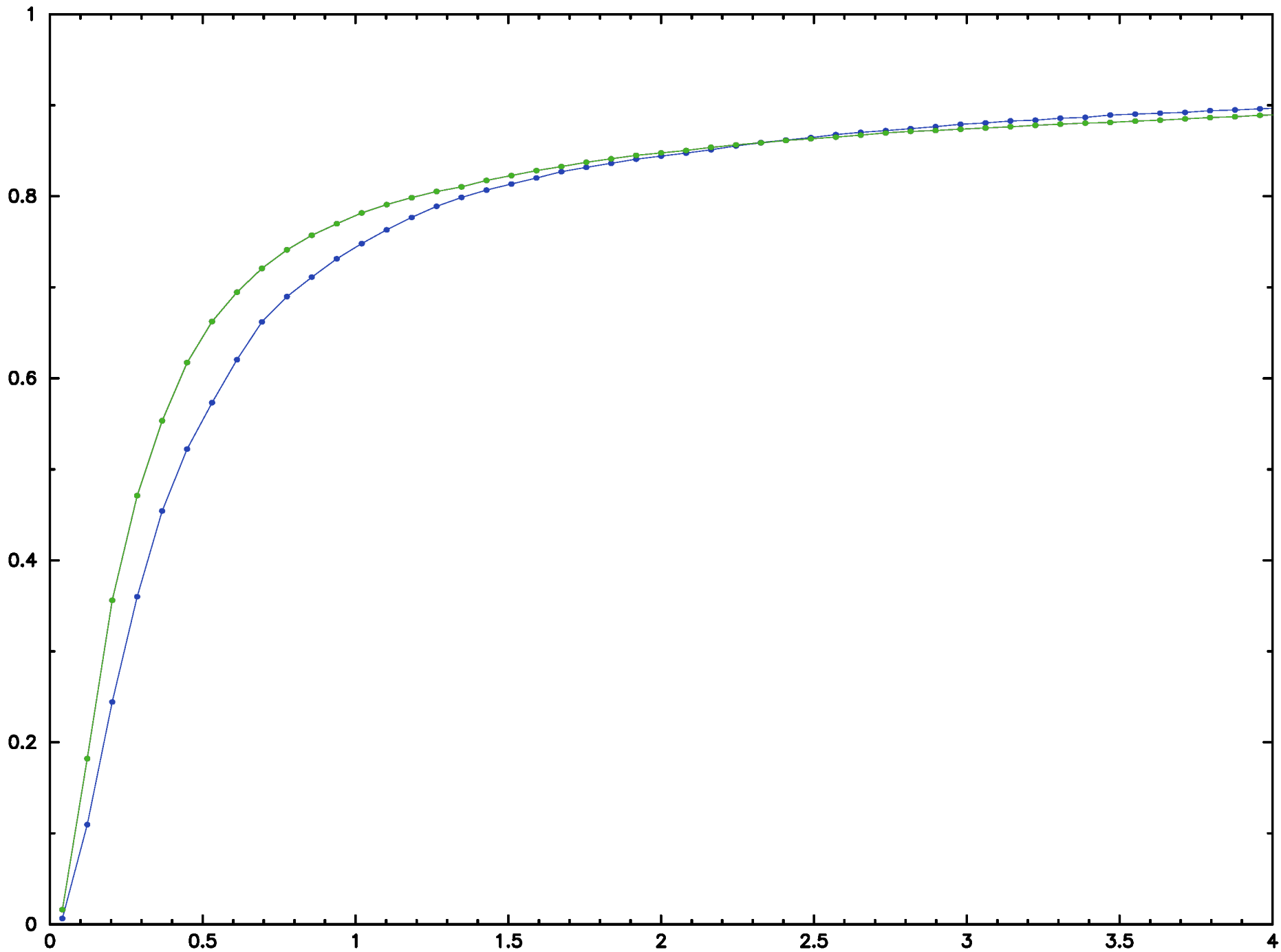
Cumulative distribution of Gaia errors
