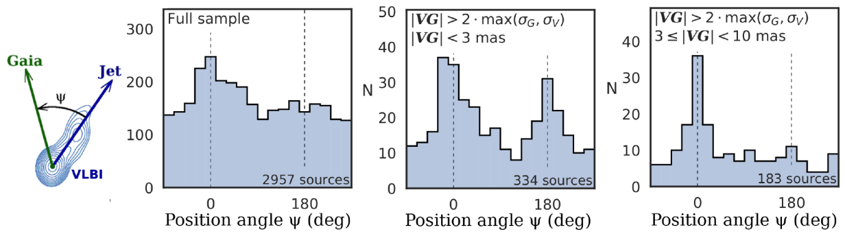
Fig. 1: The distribution of Gaia/VLBI offset directions with respect to the radio parsec-scale jet direction. Left: full sample of Gaia/VLBI matches with the probability of false association less than 2 \cdot 10^{-4} and with reliably determined jet directions. Random errors of Gaia positions are isotropic. Although random errors due to VLBI and Gaia measurement noise dominate over systematic differences due to the pretense of optical structure, we still can clearly see the signal. Center and Right: the distribution for sub-samples of Gaia/VLBI matches only with statistically significant offsets. Center: a sub-sample of position offsets less than 3 mas. Right: a sub-sample of position offsets in a range of 3–10 mas. NB: the full sample and sub-samples are not complete, they are subject of a selection bias. The goal of the proposed observations is to get rid of this selection bias. Source: Kovalev et al. (2017).
