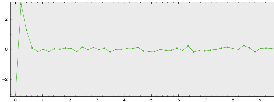
3-band I -pol fringe phase for 3C84 at MACG012M/WETTZ13S in S2081A
