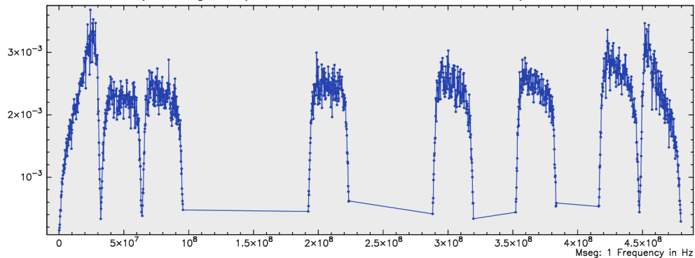
1-band I -pol fringe amplitude for 0552+398 at MACG012M/WETT13S in S2067A
