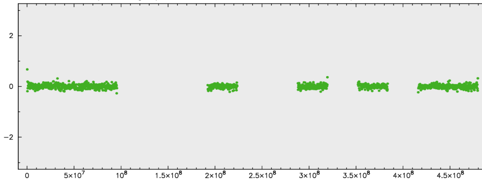
1-band I -pol fringe phase for 0552+398 at MACG012M/WETT13S in S2067A
