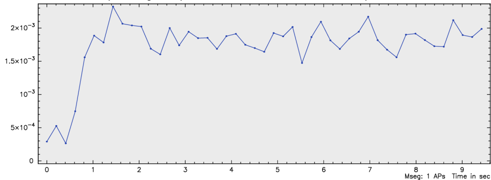
3-band I -pol fringe amplitude for 3C84 at MACG012M/WETTZ13S in S2081A
