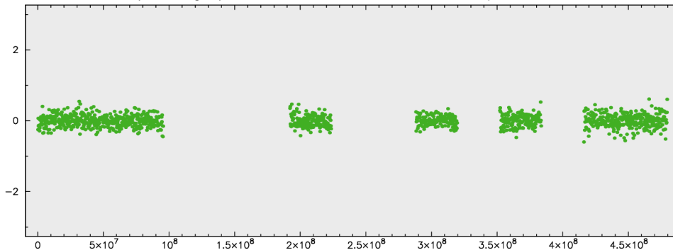
3-band I -pol fringe phase for NRA0150 at MACGO12M/WETTZ13S in S2067A
