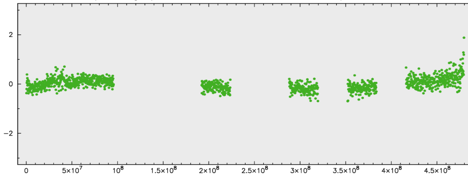
4-band I -pol fringe phase for 1803+784 at MACGO12M/WETTZ13S in S2025A
