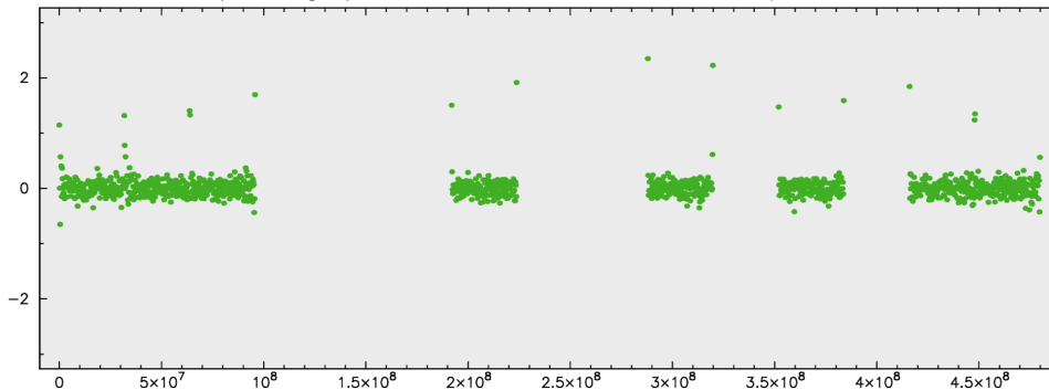
1-band HH-pol fringe phase for 0552+398 at MACG012M/WETTZ13S in S2067A
