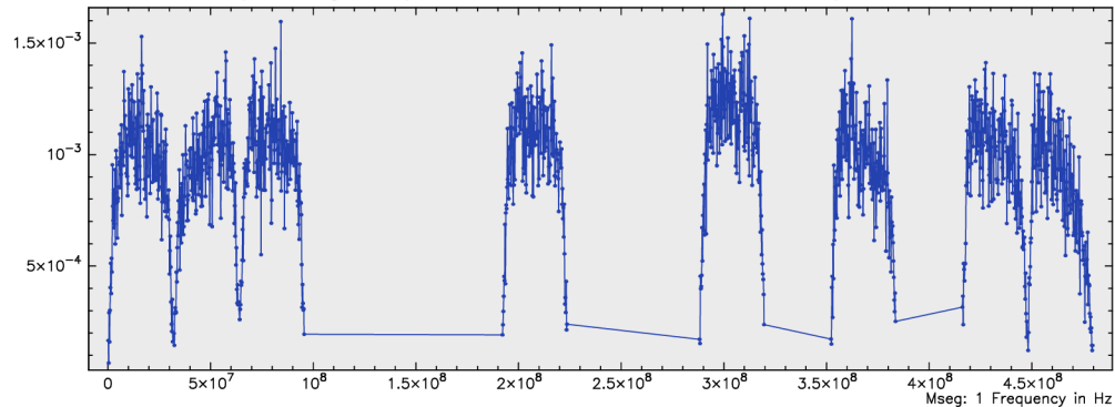
3-band I -pol fringe amplitude for NRA0150 at MACGO12M/WETTZ13S in S2067A
