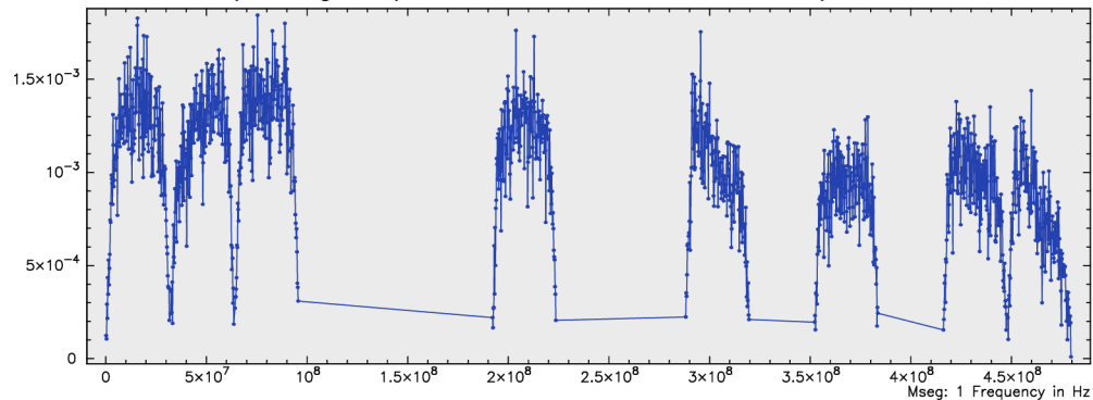
4-band I -pol fringe amplitude for 1803+784 at MACGO12M/WETTZ13S in S2025A
