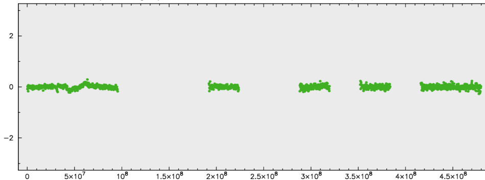
4-band I -pol fringe phase for NRA0150 at MACGO12M/WETTZ13S in S2067A
