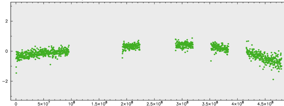
1-band I -pol fringe phase for 1803+784 at MACG012M/WETTZ13S in S2025A
