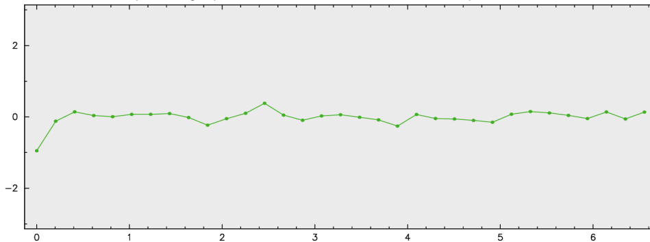
2-band I -pol fringe phase for 3C418 at MACGO12M/WETTZ13S in S2088A
