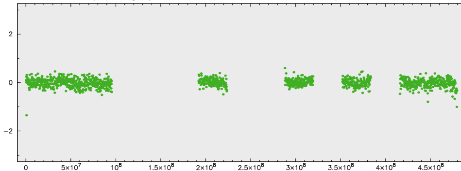
2-band I -pol fringe phase for 0552+398 at MACG012M/WETT13S in S2067A
