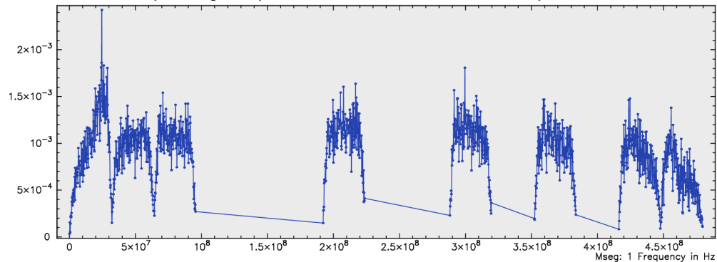
1-band I -pol fringe amplitude for 1803+784 at MACG012M/WETTZ13S in S2025A
