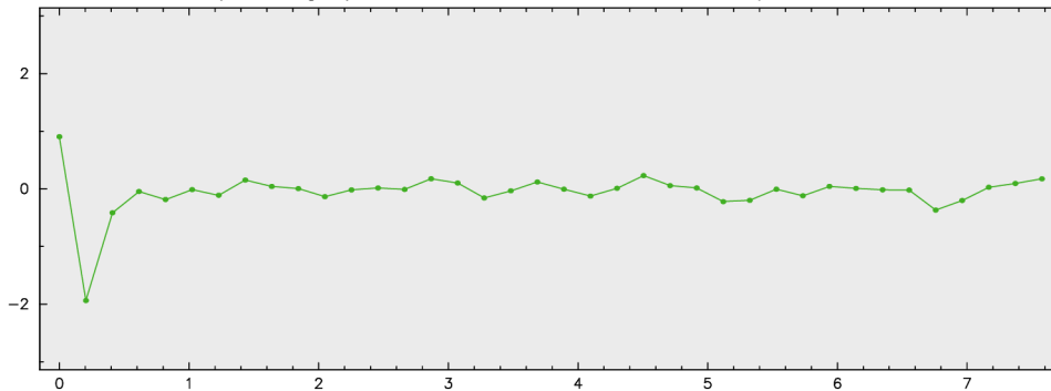
2-band I -pol fringe phase for 3C418 at MACG012M/WETTZ13S in S2088A
