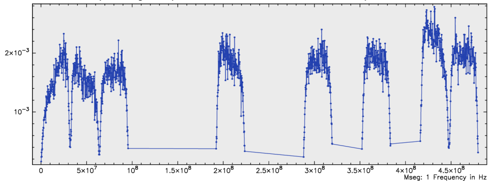
1-band I -pol fringe amplitude for 0420-014 at MACG012M/WETT13S in S2053A
