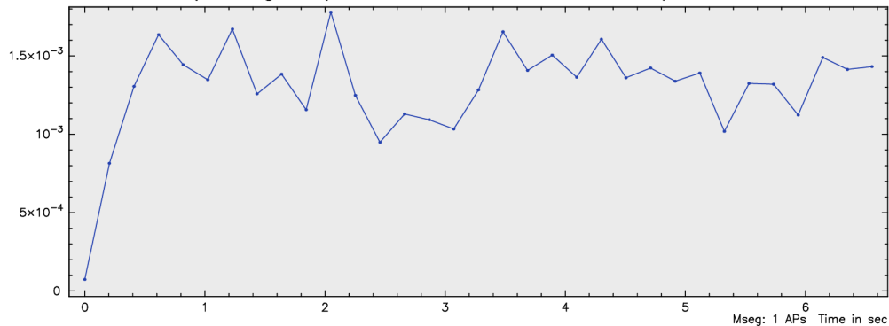
2-band I -pol fringe amplitude for 3C418 at MACGO12M/WETTZ13S in S2088A
