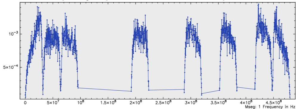
1-band HH-pol fringe amplitude for 0552+398 at MACG012M/WETTZ13S in S2067A
