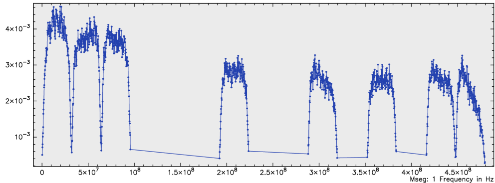
4-band I -pol fringe amplitude for NRA0150 at MACGO12M/WETTZ13S in S2067A
