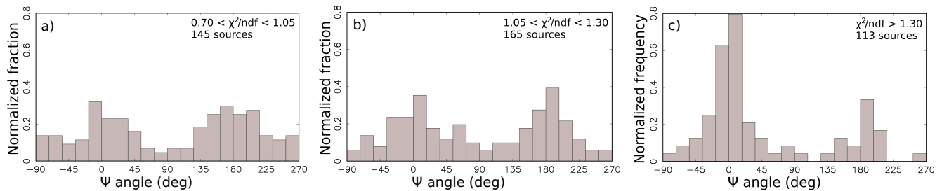
Figure 7. The histograms of the distribution of the position angle of Gaia offset with respect to VLBI positions for matches with \sigma_{\psi} < 0.3 rad and arc-lengths < 2.5 mas and different ranges of \chi^2/\text{ndf} .
