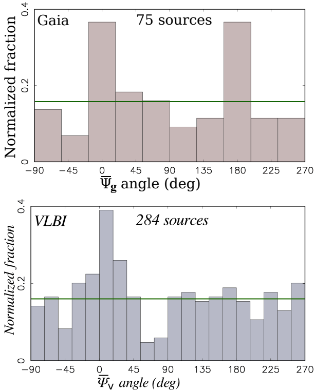
Figure 8. The histograms of significant AGNs proper motion position angles with respect to jet directions among matching sources \Psi_g for Gaia and \Psi_v for VLBI. Up: the Gaia DR2 proper motions with magnitudes > 3\sigma in both proper motions and position offsets. Down: the proper motions from the VLBI global solution. The horizontal green line shows the uniform distribution.
