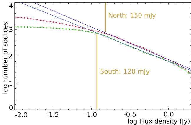
Figure 13. The log N–log S diagram for the LCS catalogue (low green line) using only the sources with \delta < -40^\circ . The upper red line shows similar diagram for the sources with \delta > +40^\circ .
