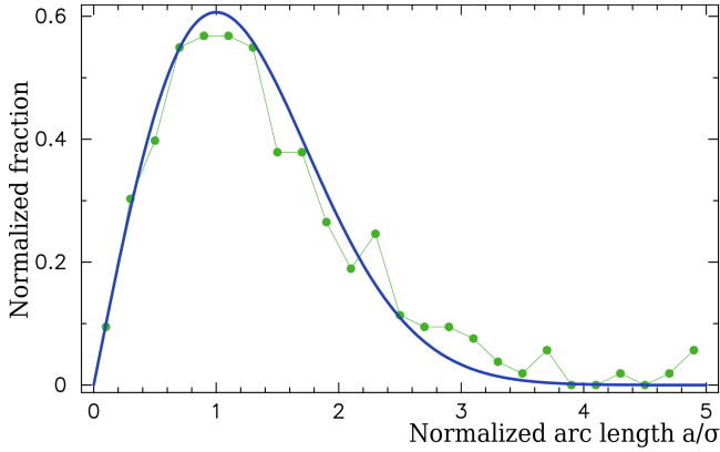
Figure 9. The distribution of the normalized arc lengths between LCS X-band only positions of 269 sources and their X/S positions from the follow-up campaigns (Green dots). For comparison, the Rayleigh distribution with \sigma = 1 parameter is shown with a blue line.
