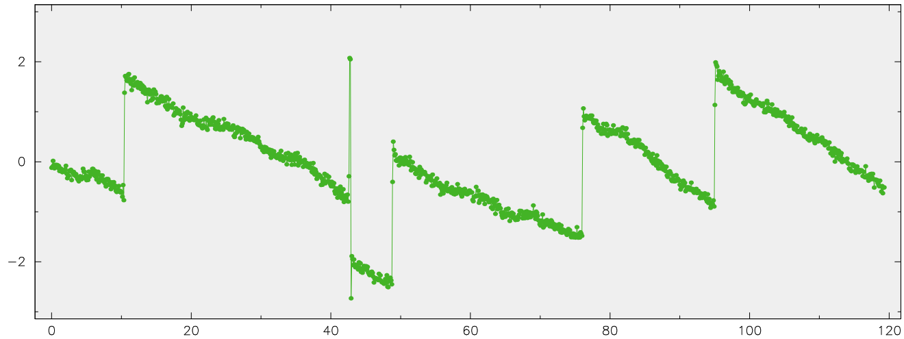
Q-band I -pol fringe phase for 1546+027 at KVNUS /KVNYS in N20LP01
