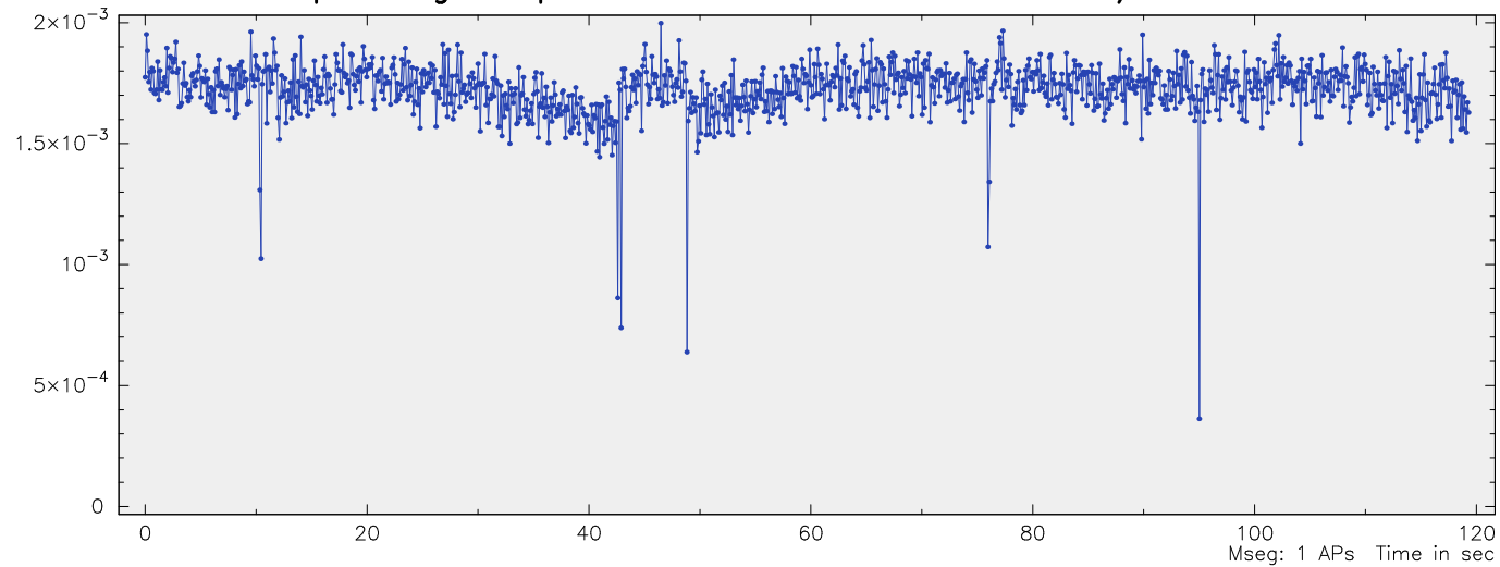
Q-band I -pol fringe amplitude for 1546+027 at KVNUS /KVNYS in N20LP01
