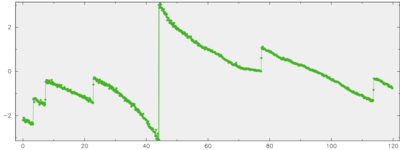
K-band I -pol fringe phase for 3C273B at KVNUS /KVNYS in N20LP01
