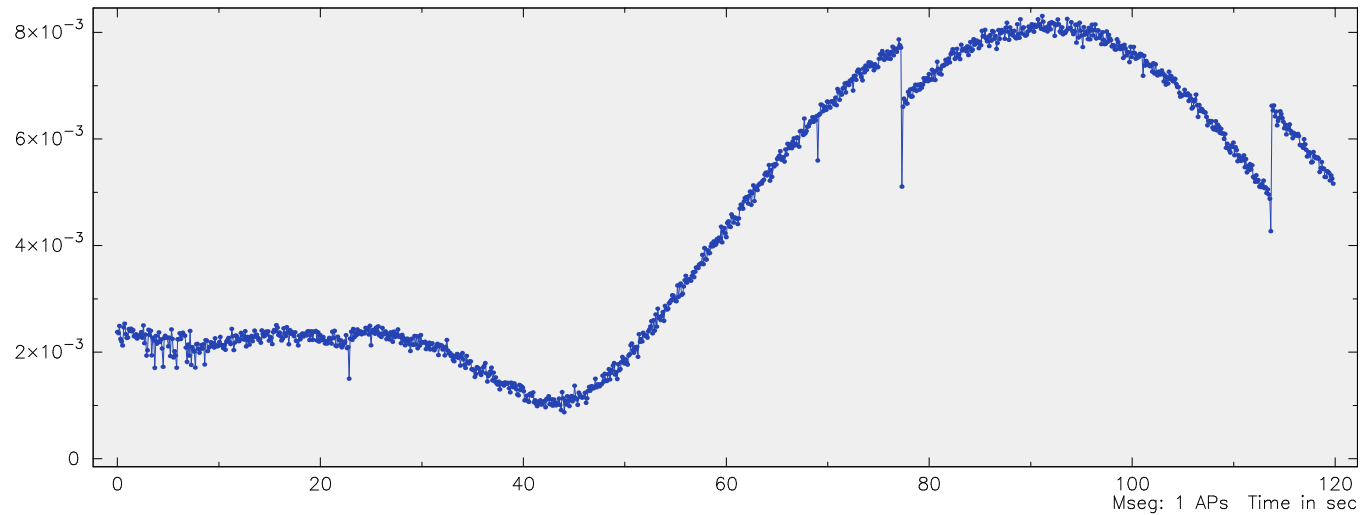
K-band I -pol fringe amplitude for 3C273B at KVNUS /KVNYS in N20LP01
