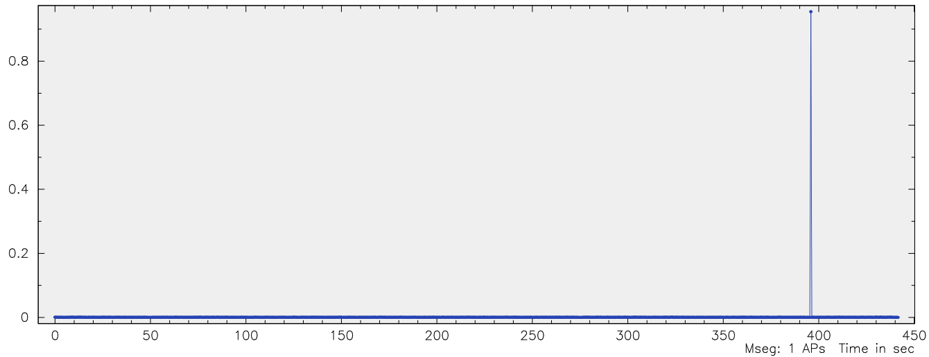
X-band fringe amplitude for 1532+824 at LA-VLBA /OV-VLBA in BK130
