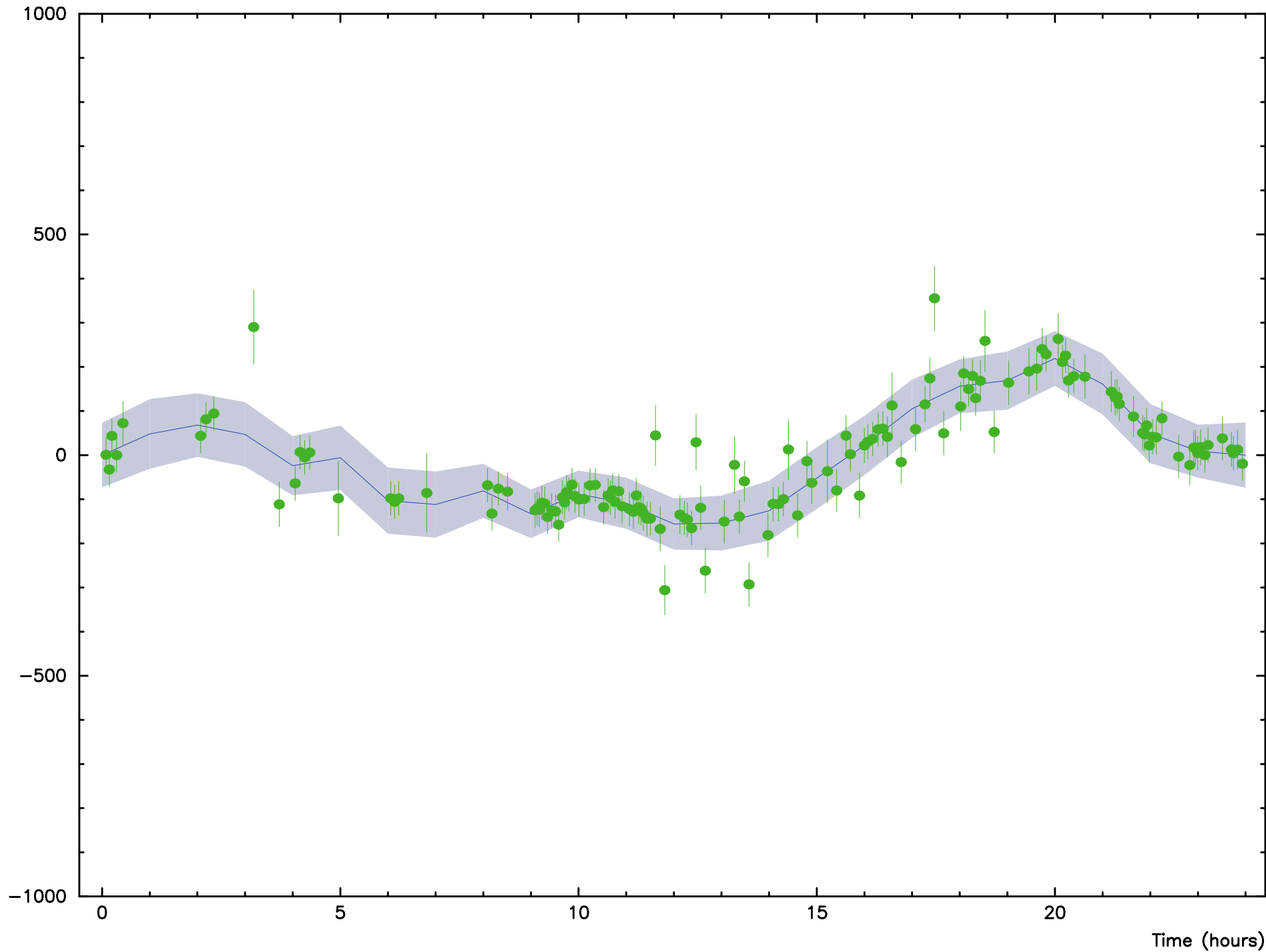
20191128_s <2> HARTRAO/MEDICINA Residuals + clock wrms=39.5 ps
