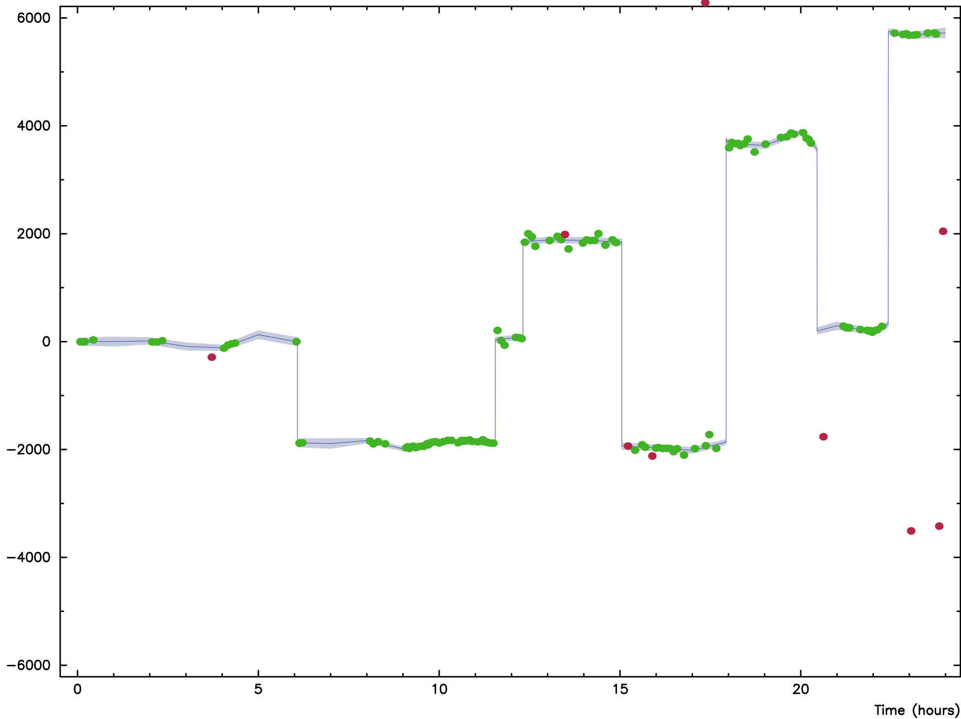
20191128_b <1> HARTRAO/MEDICINA Residuals + clock wrms=22.0 ps
