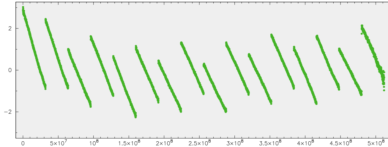
X-band LL-pol fringe phase for 4C39.25 at RAEGYEB /YEBES40M in RU0829
