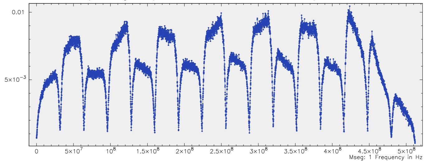
X-band LL-pol fringe amplitude for 4C39.25 at RAEGYEB /YEBES40M in RU0829
