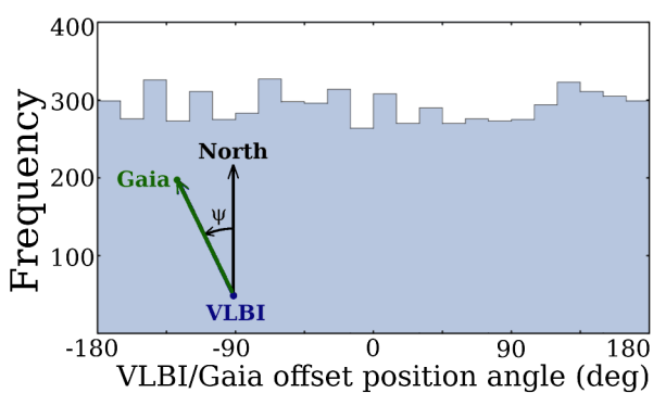
Figure 2: Left: the distribution of VLBI/Gaia position offsets with respect to the north direction. Right: the distribution of AGN jet directions measured with VLBI with respect to the north direction.
