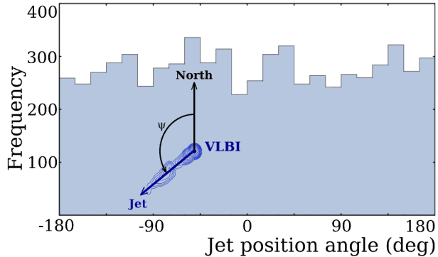
Figure 2: Left: the distribution of VLBI/Gaia position offsets with respect to the north direction. Right: the distribution of AGN jet directions measured with VLBI with respect to the north direction.
