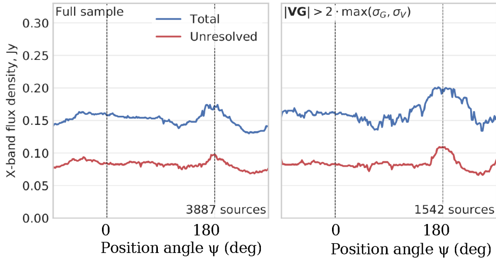
Figure 7: The histogram of the dependences of flux density at 8 GHz of VLBI/ Gaia matches as a function of the Gaia position offset \psi with respect to jet direction. The total flux density is integrated over the image and is confined to 10 mas area. The unresolved flux density characterizes the radio flux density at sub-mas scales. Left : full sample. Right : sub-sample of statistically significant offsets. The histogram was smoothed with the moving median with \pm 50^\circ window.
