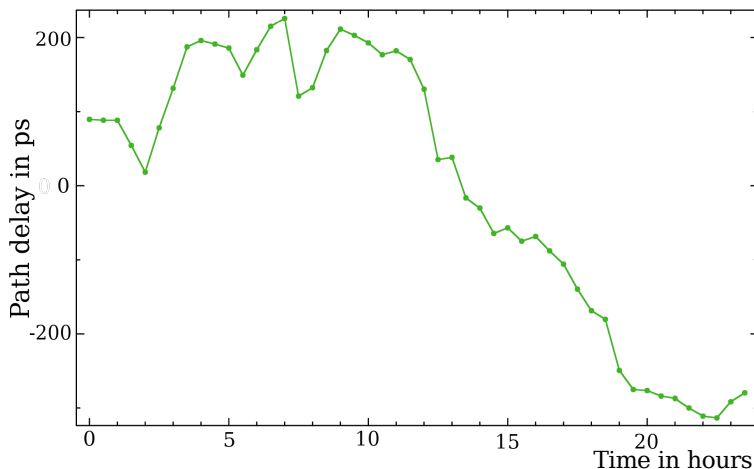
Figure 3: Variation of moist (dry and wet) path delay in zenith direction for station GGAO12M (suburb of Washington DC) with respect to the average value 8157 ps on 2006.01.01 computed using the output of GMAO 7km Nature Run.
